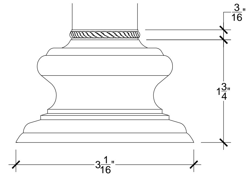
New Base Detail Scale 1:1
